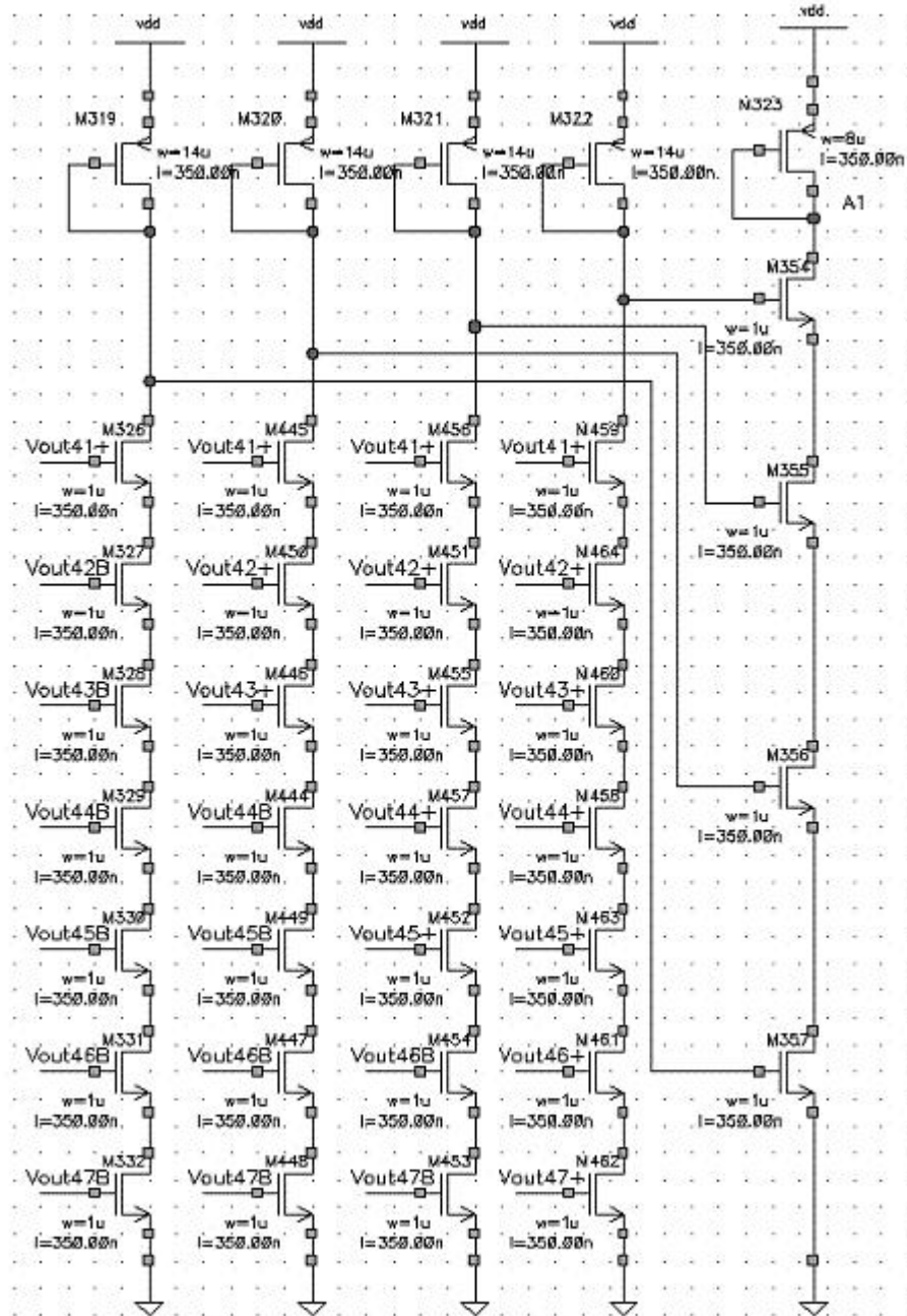
Fig. 3.14. Digital encoder circuit for bit A1.
