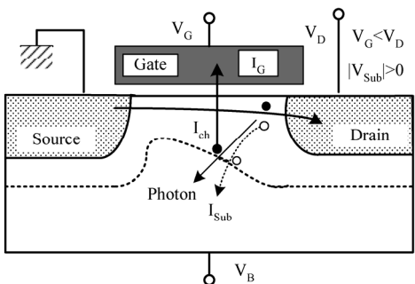
Fig. 2.6. Secondarily generated hot electron injection
